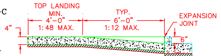
MIN 2" D.G.A. SECTION B-B
