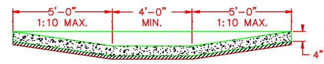
MIN 2" D.G.A. SECTION C-C
