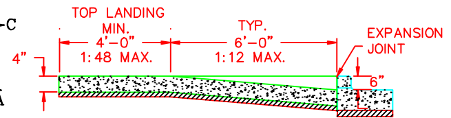
MIN 2" D.G.A. SECTION B-B
