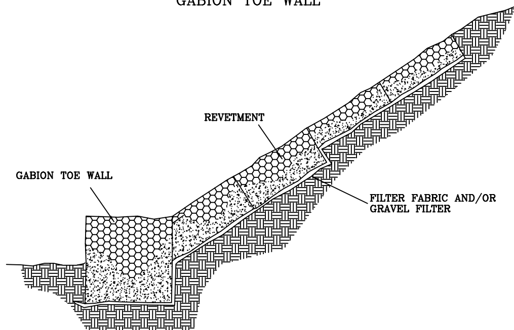
GABION TOE WALL
