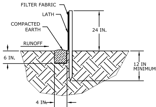
FLAT BOTTOM TRENCH SECTION
