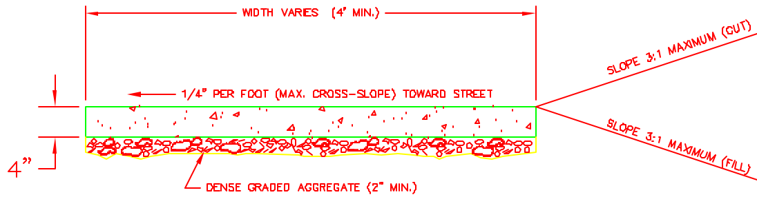
SIDEWALK DETAIL (TYPICAL SECTION) (N.T.S)
